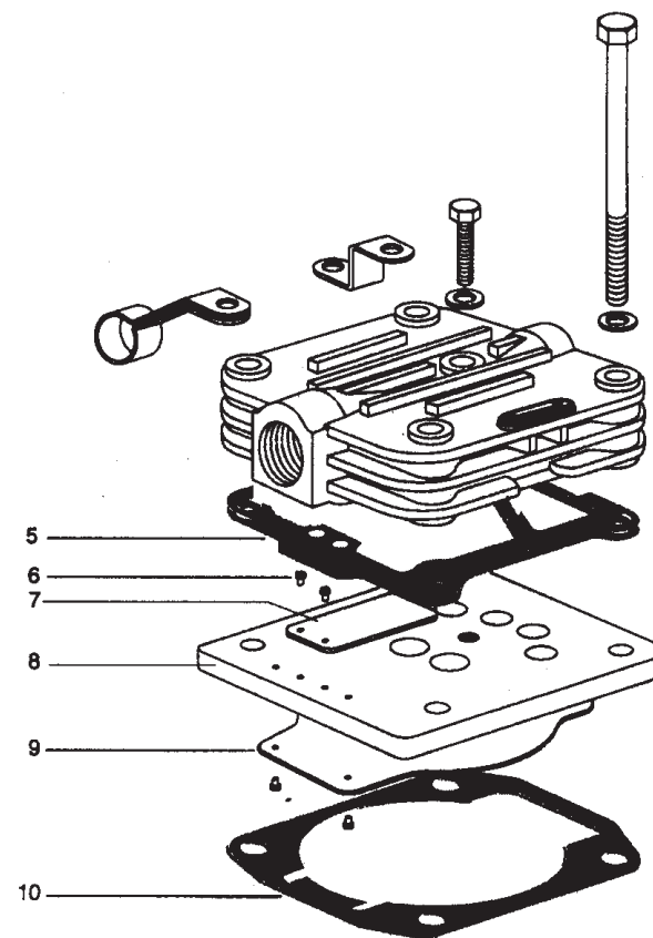
AIR COMPRESSOR HEAD (REED VALVE TYPE) 94 DIA
