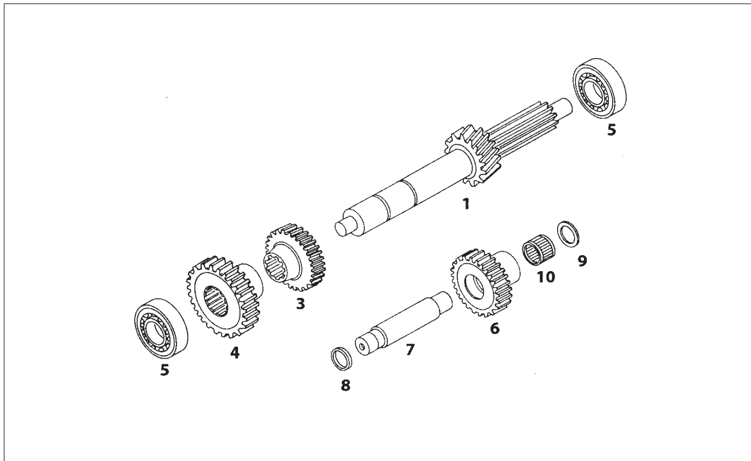
COUNTER SHAFT, GEARS AND REVERSE IDLER
