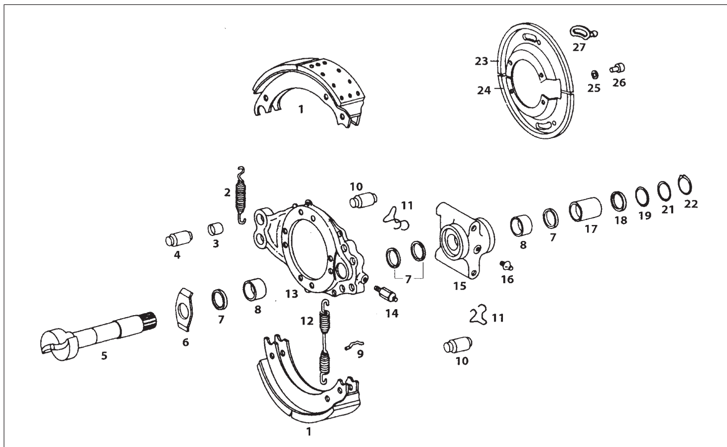
REAR WHEEL BRAKE (M/S AAL) -- LP
