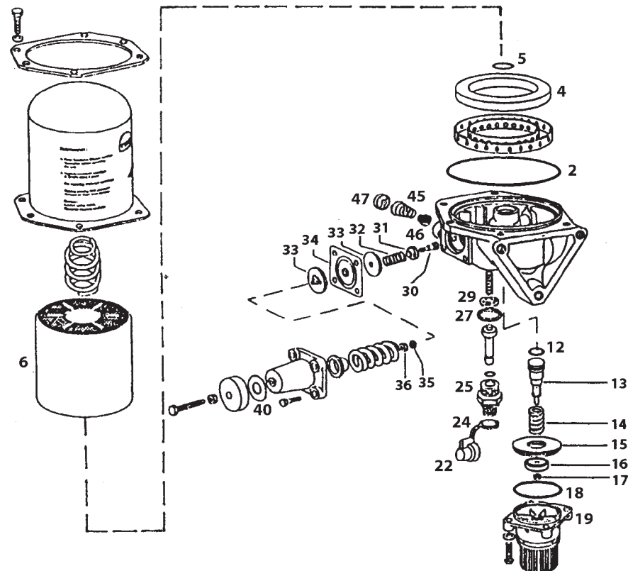
AIR DRYER WITH TYRE INFLATOR
